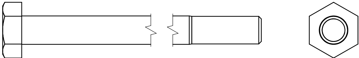
(A7)HEX BOLT 1/2"x6"L PARTIAL THREAD QTY.1
