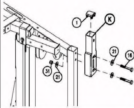
REVERSE SIDE DRAWING
